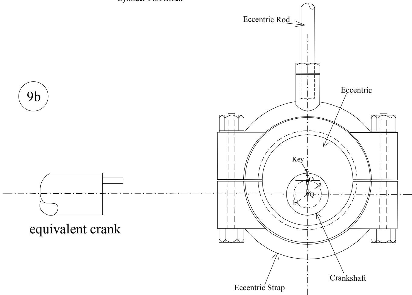
Fig 9 Details of slide valve and eccentric
