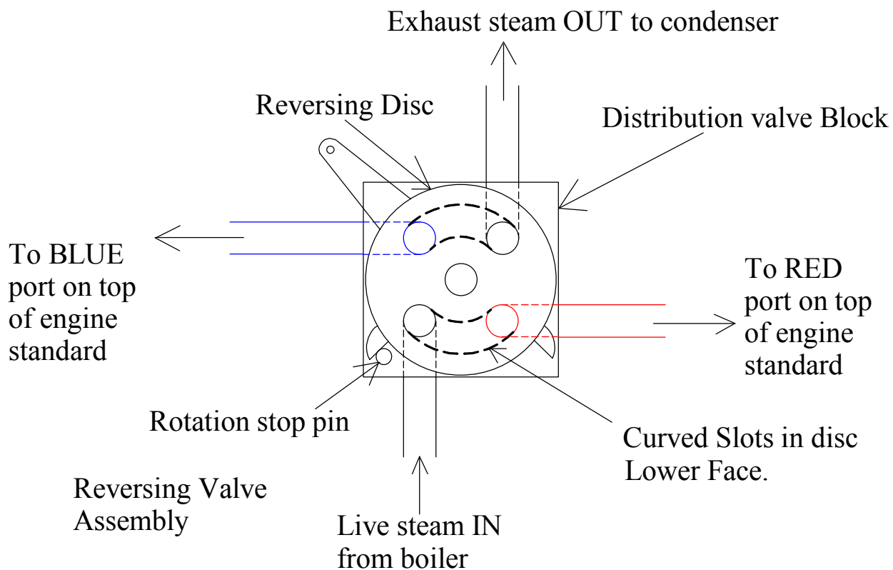
Fig 7.1 Oscillating engine.
