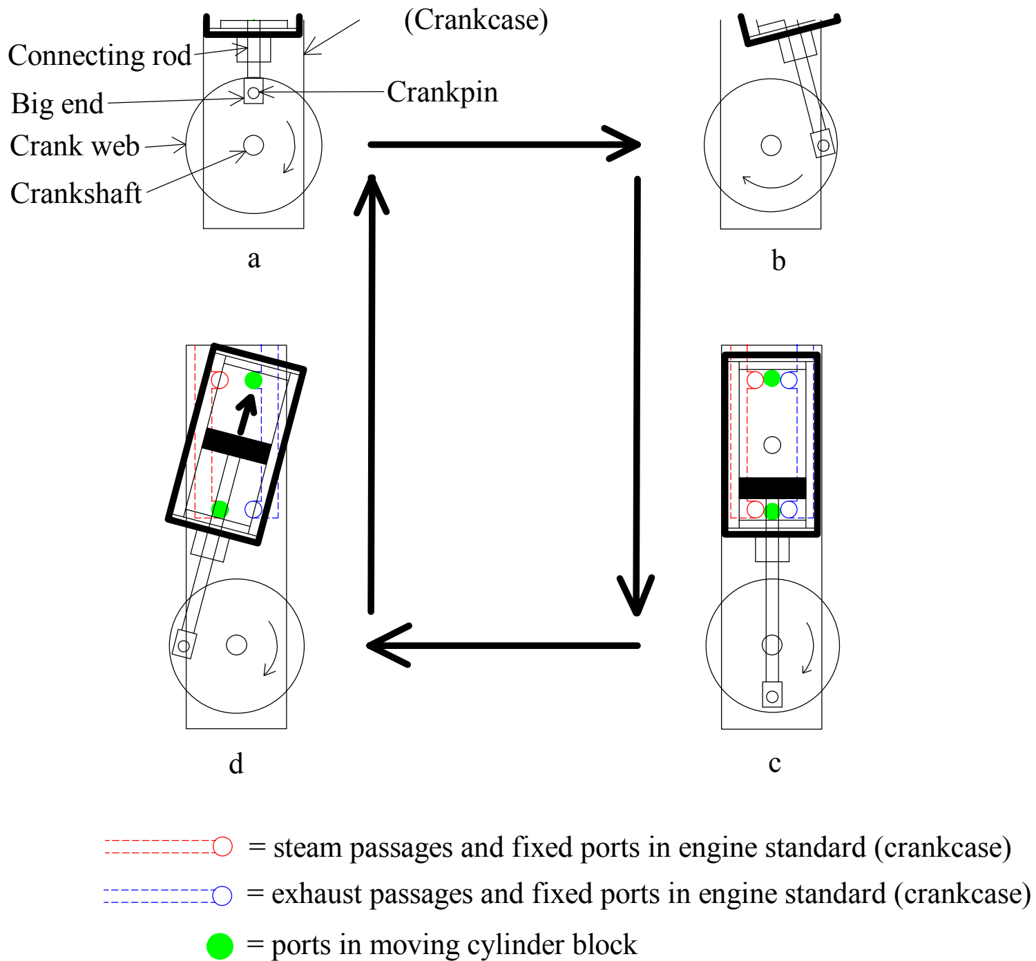
Fig 7.2 Oscillating engine sequence.
