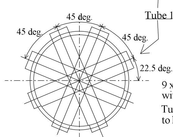
View on burner end of centre flue
