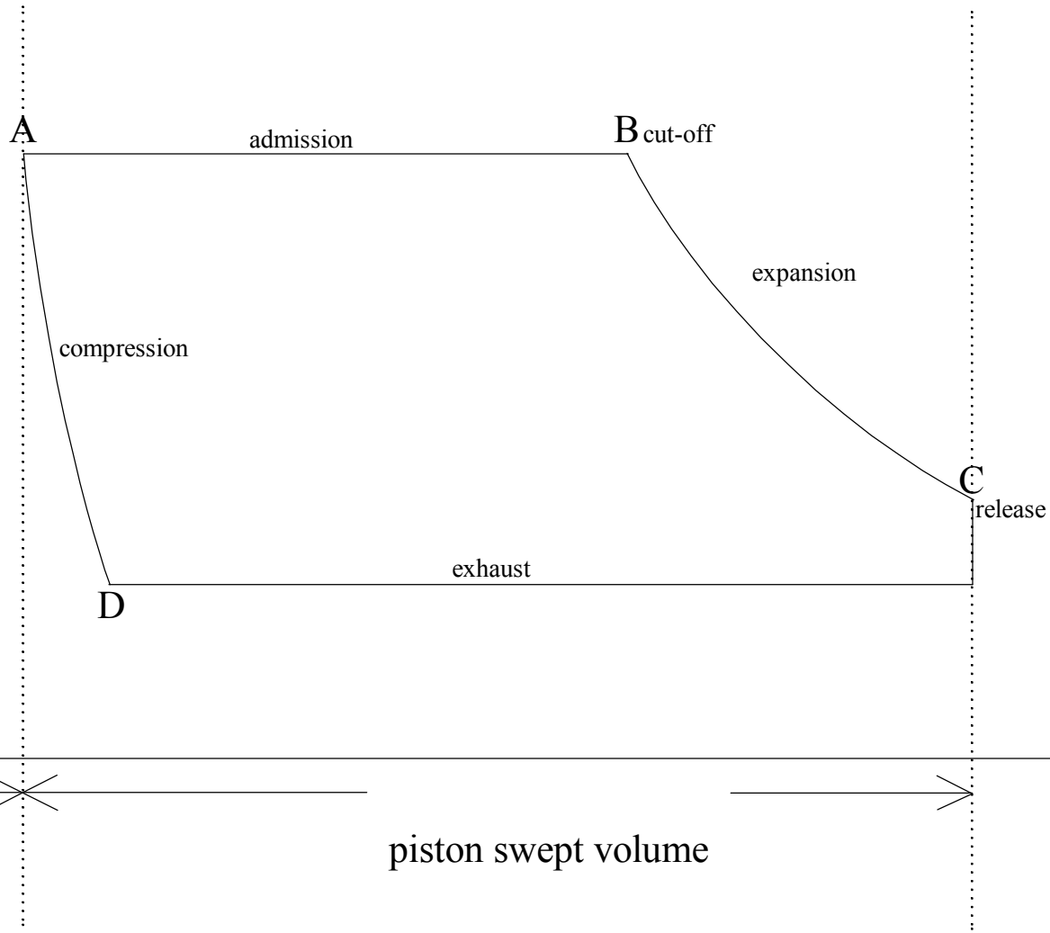
Fig 4 Hypothetical indicator diagram
