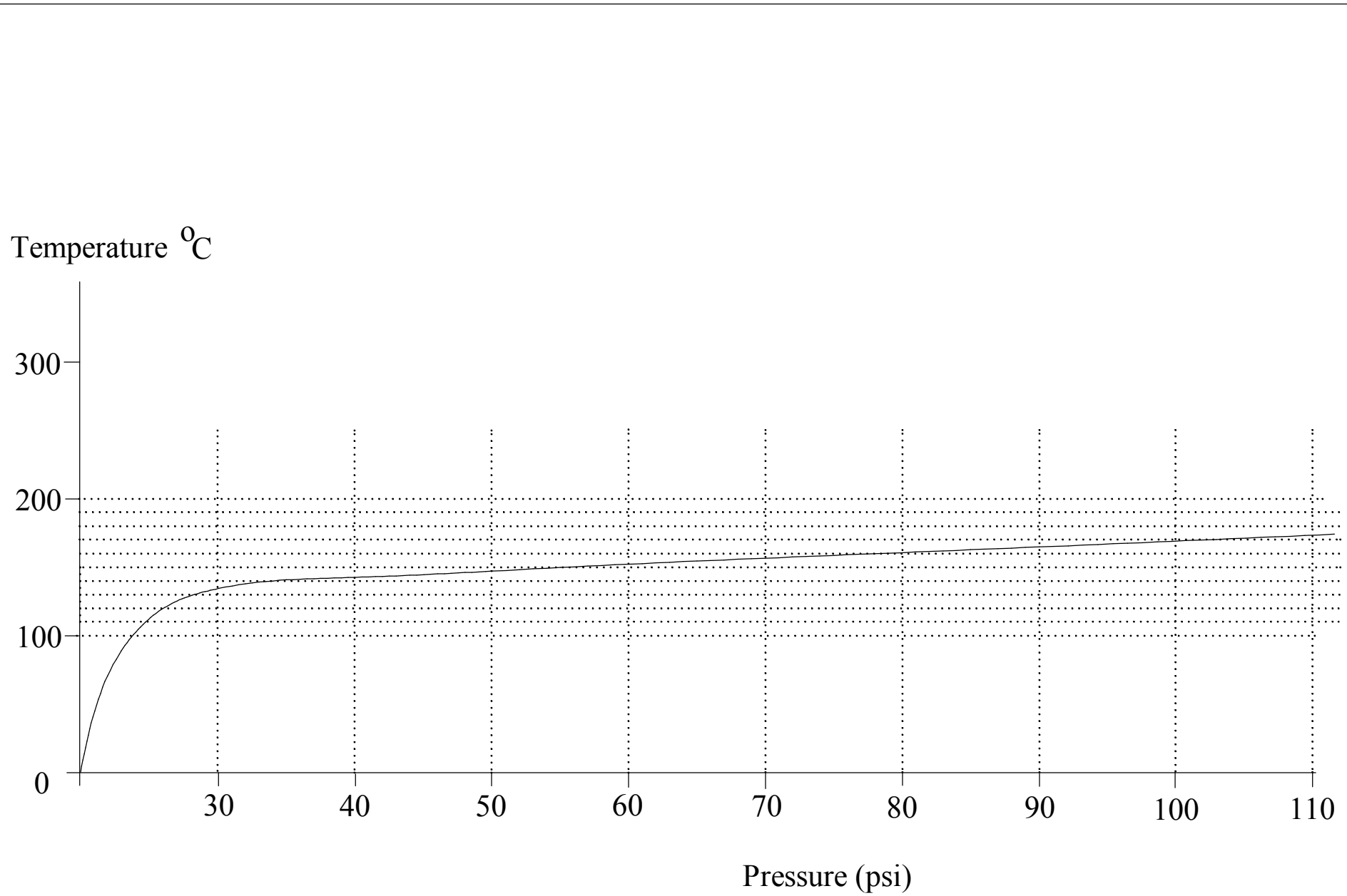
Fig 1 Saturated Steam Pressure V Temperature
